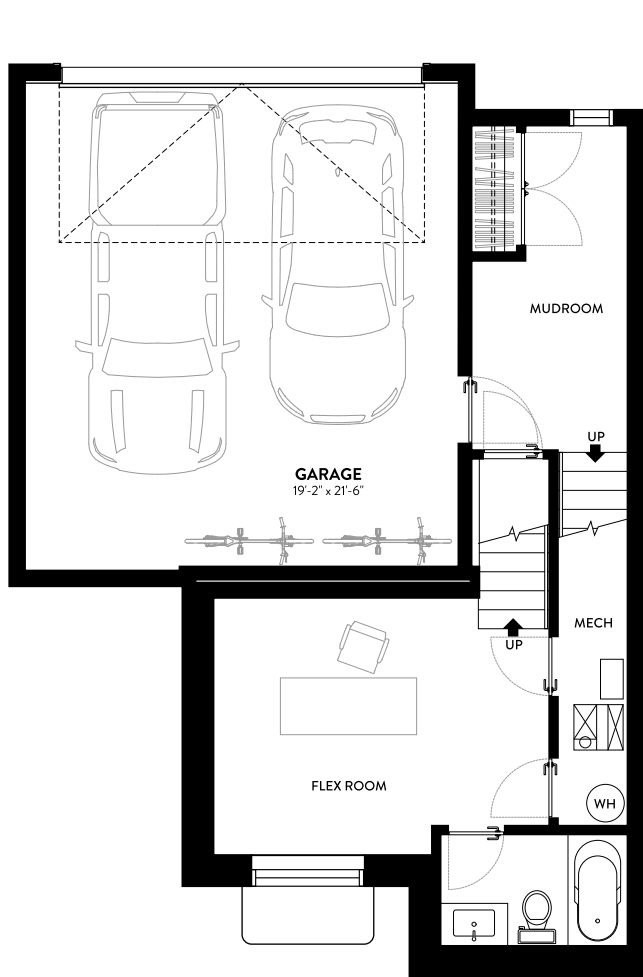
LOWER LEVEL 157 SQ.FT. OPTIONAL DEVELOPMENT 278 SQ.FT.
