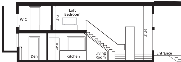
Side Elevation
