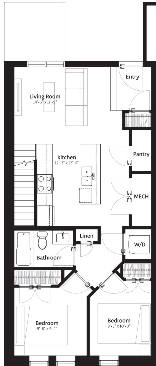
MAIN 813 SQ.FT.
