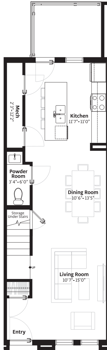
MAIN 605 SQ.FT.
