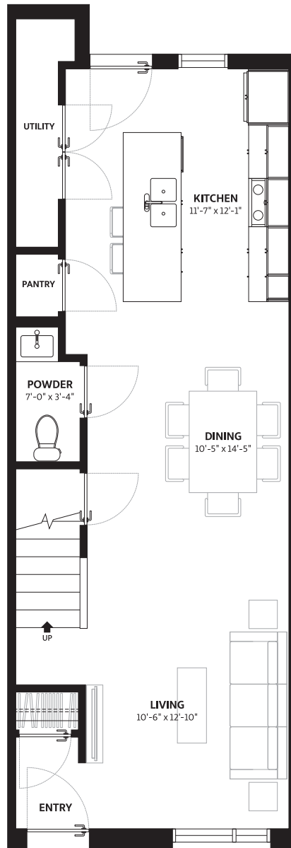
MAIN 615 SQ.FT.
