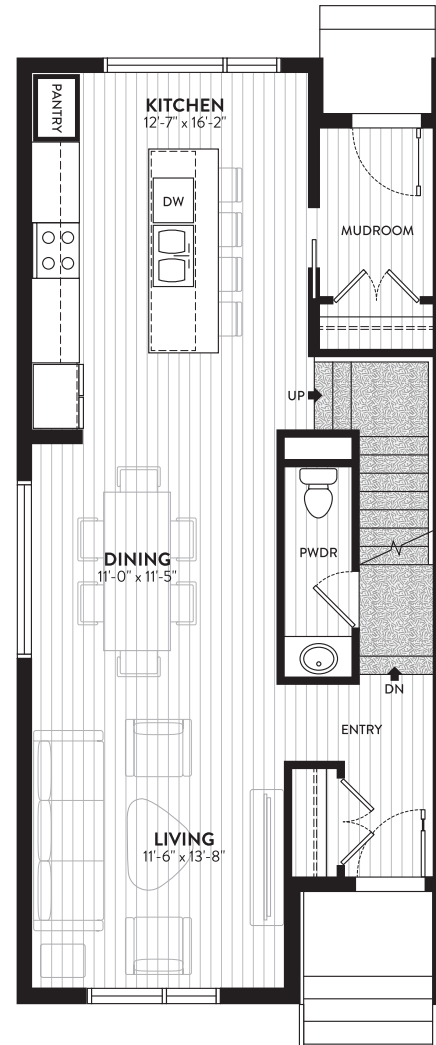
MAIN FLOOR 757 SQ.FT.
