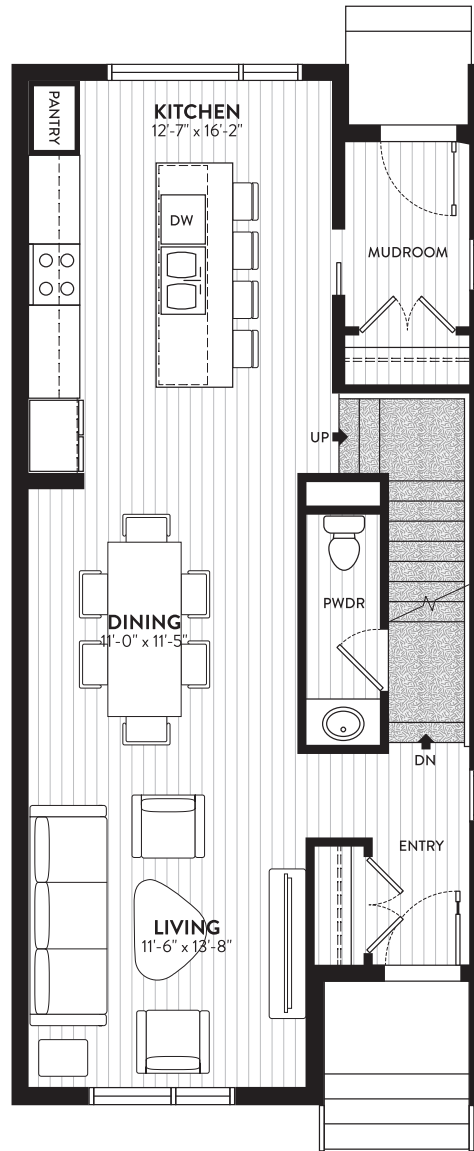
MAIN FLOOR 756 SQ.FT.
